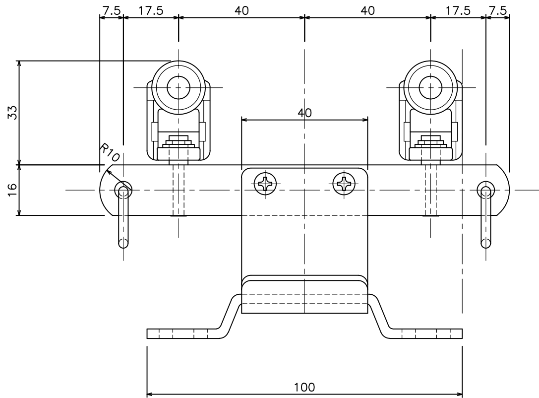
吊り金具C (15Y63)
