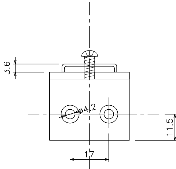
紐留め金具 (76T82)
